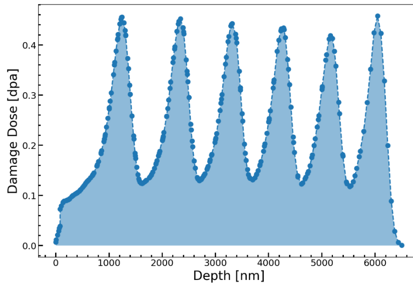
Figure 9: Combined damage dose plot for different thicknesses of an Al foil on a Cu layer under 3.25 MeV He irradiation. Fluence = 6.7e15 , reference layer = 2 (depth refers to depth into Cu layer).
